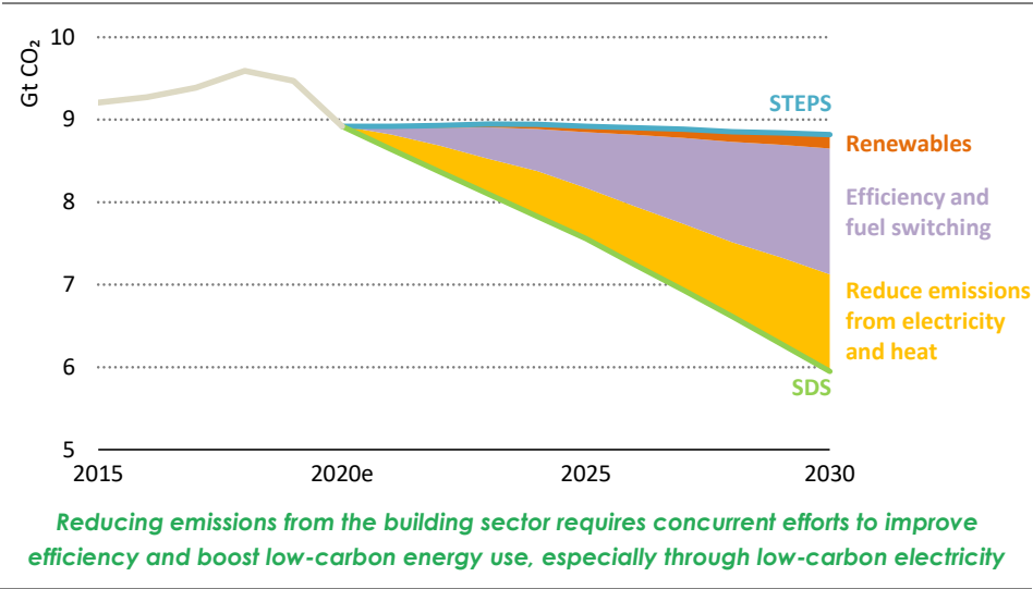
Figure 3.16 ▶ Direct and indirect CO 2 emissions in buildings in the Stated Policies and the Sustainable Development scenarios
