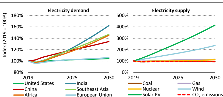
Figure 6.1 ▶ Electricity outlook in the Stated Policies Scenario, 2019-2030
