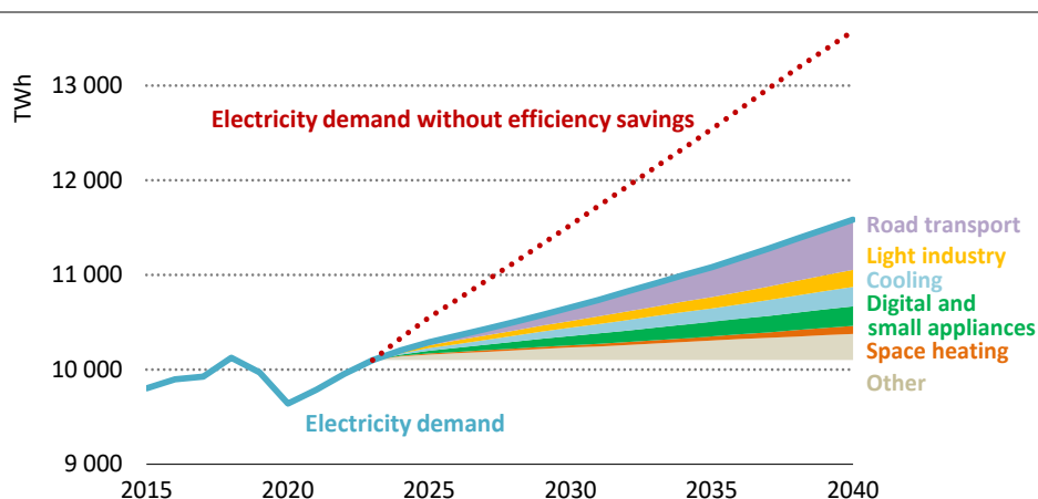
Figure 6.6 ▶ Drivers of electricity demand in advanced economies in the Stated Policies Scenario
