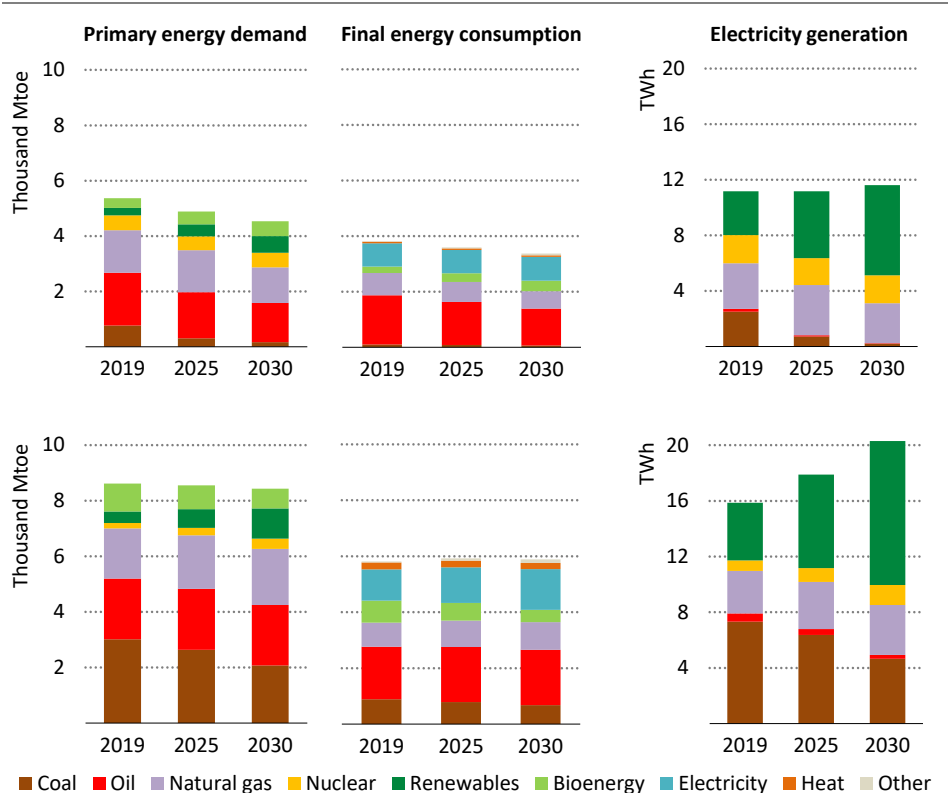
Figure 3.10 ▶ Energy sector transformation in advanced economies (top) and emerging market and developing economies (bottom)
