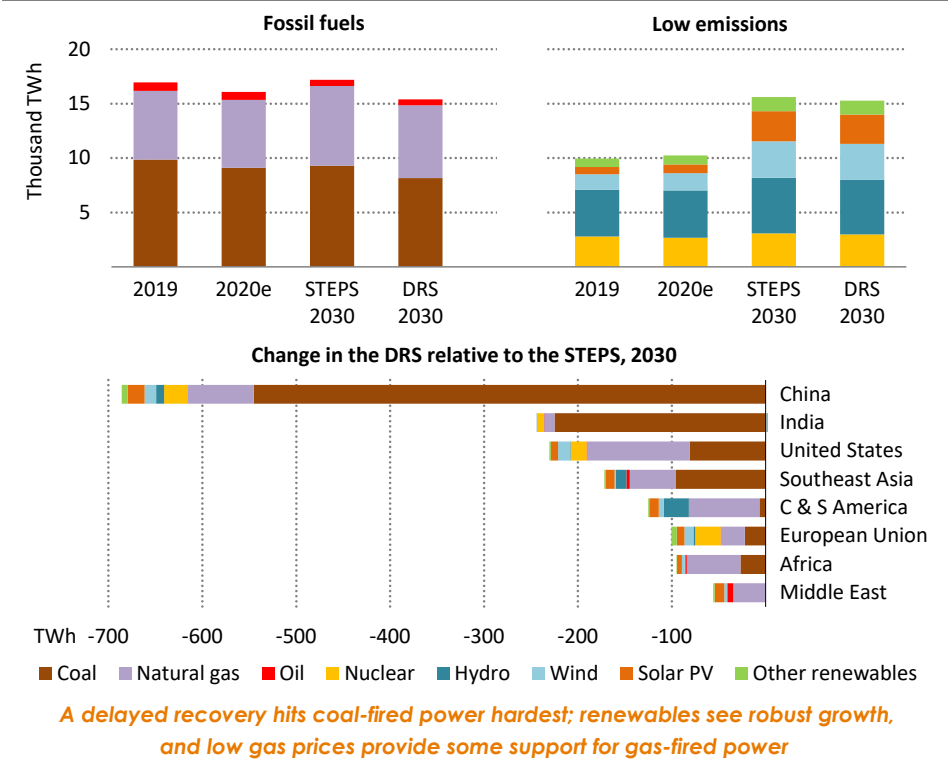
Figure 8.8 ▶ Electricity generation mix in the Delayed Recovery Scenario relative to the Stated Policies Scenario
