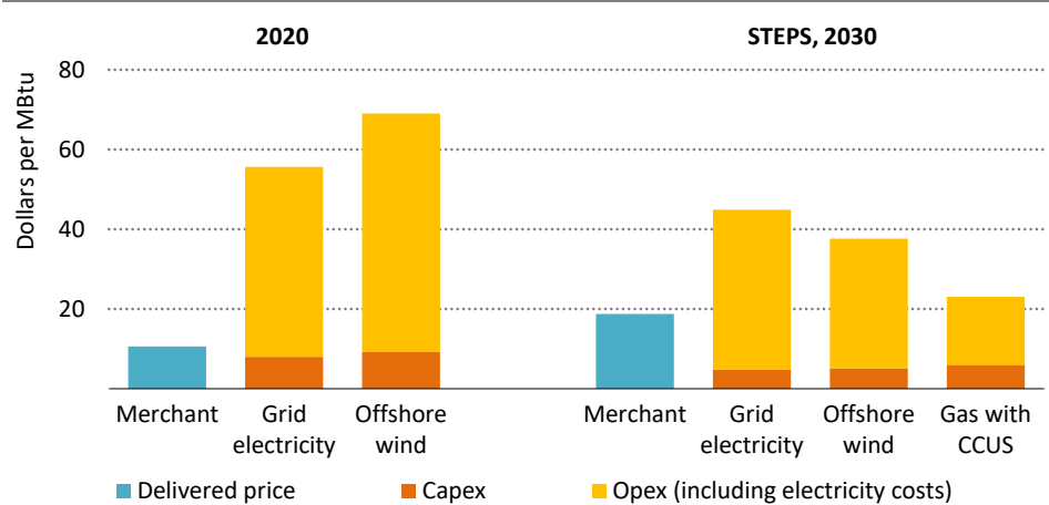
Figure 7.21 ▶ Cost gap to be bridged between the costs of delivered low-carbon and merchant hydrogen in Europe, 2020 and 2030
