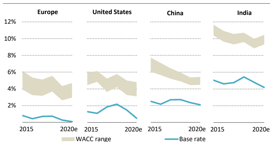
Figure 6.15 ▶ Indicative WACC for utility-scale solar PV projects with revenue support
