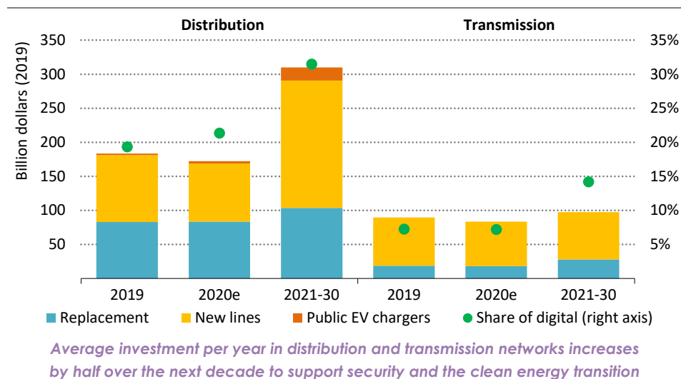
Figure 6.19 ▶ Annual investment in electricity networks by sector in the Stated Policies Scenario
