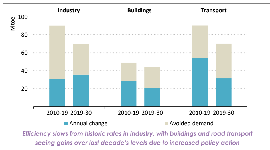
Figure 5.23 ▶ Average annual change in energy consumption and avoided demand due to efficiency improvements by sector in the Stated Policies Scenario
