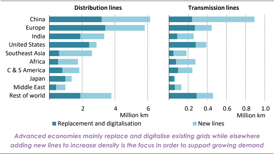
Figure 6.18 ▶ Length of new and replaced electricity network lines by selected region in the Stated Policies Scenario, 2019-2030
