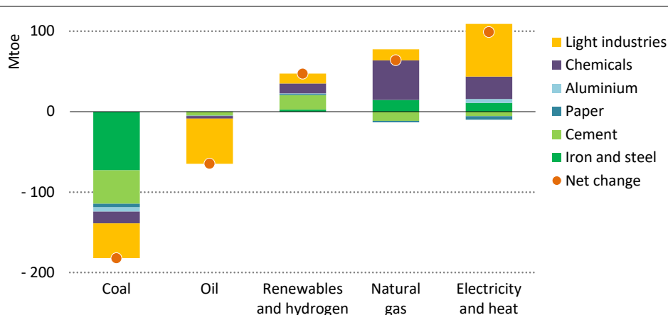
Figure 3.14 ► Changes in fuel consumption for energy and feedstock use in industry in the Sustainable Development Scenario, 2019-2030
